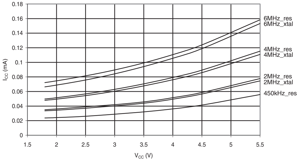
Figure 31-108. ATmega88A: Standby Supply Current vs. V_{CC} (Watchdog Timer Disabled)
