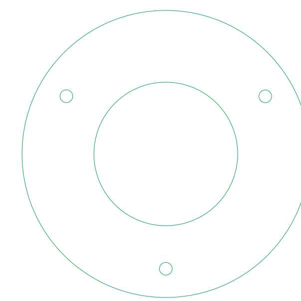
MOTOR MOUNT RETAINER 1/8" BIRCH PLYWOOD
