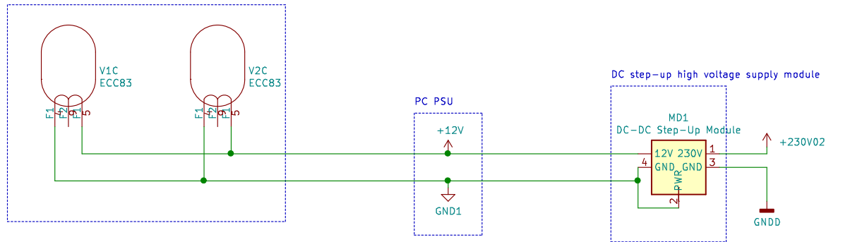
Filament voltage supply pattern
