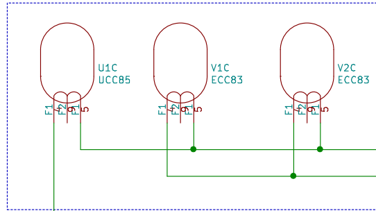
Filament voltage supply pattern
