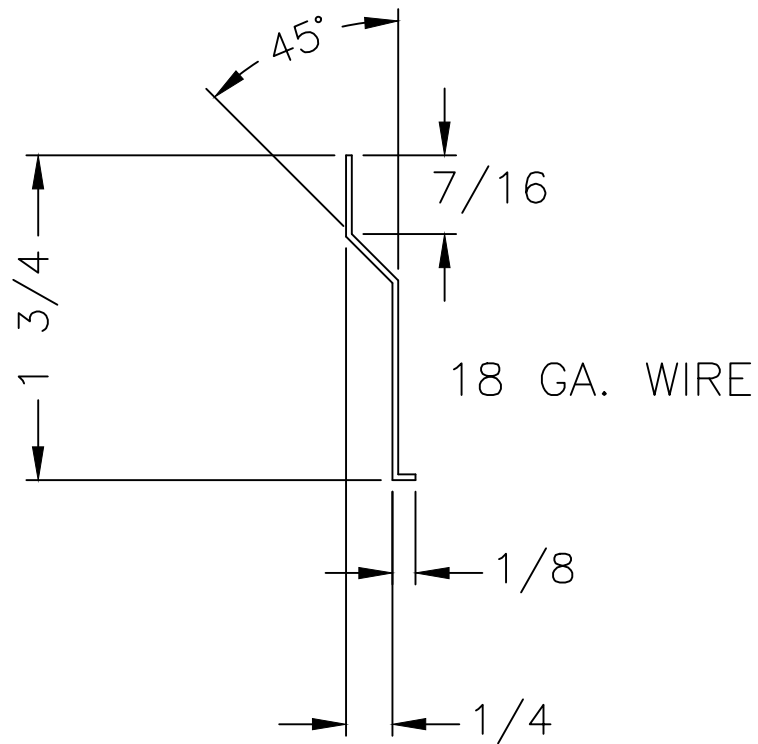
MOON SUPPORT
