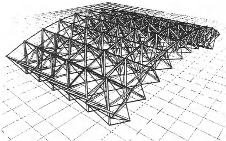
Figure 4.50 Single curvature double layer tensegrity grid
