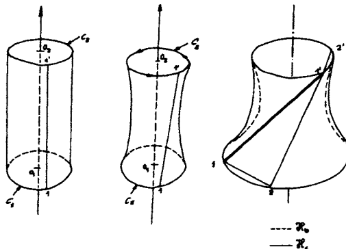
Figure 4.8 Generating hyperboloids
