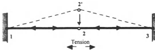
Figure 5.24 Tension pre-stress
