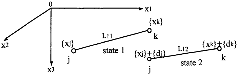
Figure 6.36 Displacement increments
