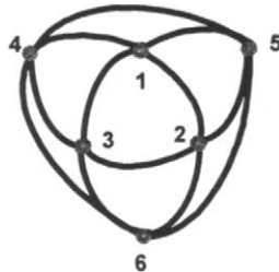
Figure 3.1 Six nodes complete plane graph
