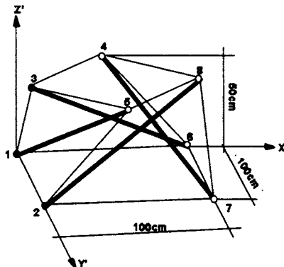
Figure 5.35 Quadruplex
