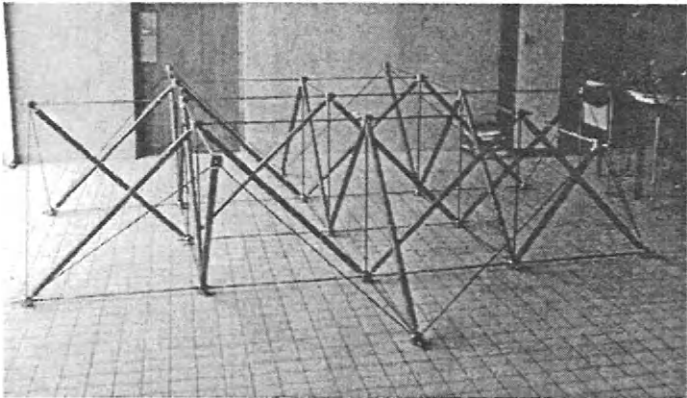
Figure 7.13 “Mini grid”
