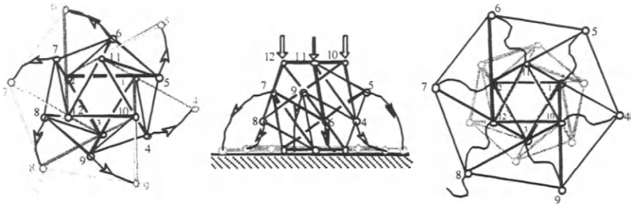
Figure 6.17 Nodes trajectories
