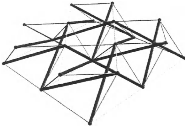
Figure 2.19 Complete grid
