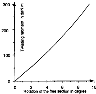
Figure 5.38 Torsion
