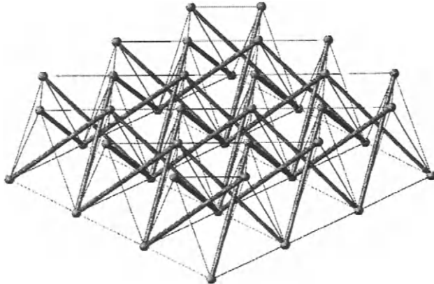
Figure 7.2 Double layer tensegrity grid: axonometric view
