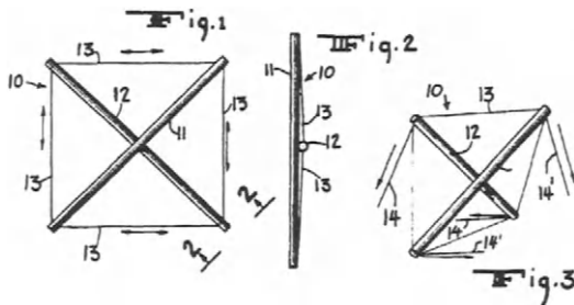
Figure 2.8 Kenneth Snelson: Continuous Tension, Discontinuous Compression. Basic concept
