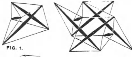
Figure 2.2 Emmerich's patent
