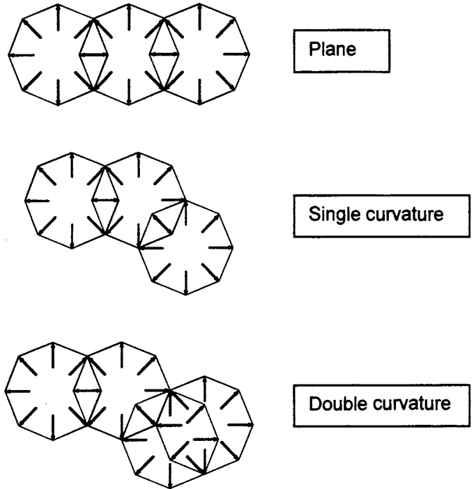
Figure 2.17 Structural situation diagrams
