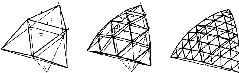
Figure 4.15 Breakdown frequency
