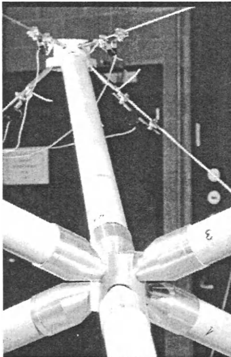
Figure 7.32 Central node
