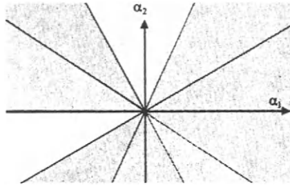
Figure 5.32 No feasible self-stress
