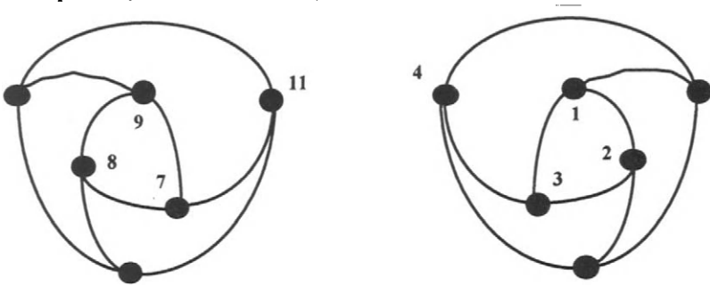
Figure 6.4 Cable graphs of three-strut tensegrity systems
