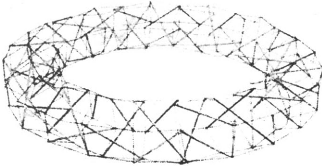
Figure 4.31 Tensegrity "torus"
