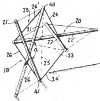
Figure 5.5 Assembling two “X”
