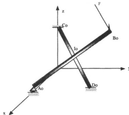
Figure 6.37 Two struts in contact. Initial configuration ( \Gamma_0 )
