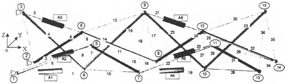
Figure 5.48 Tensegrity beam
