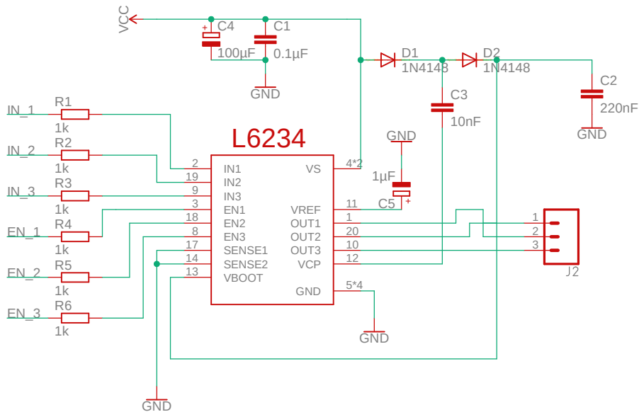
L6234 three phase motor driver
