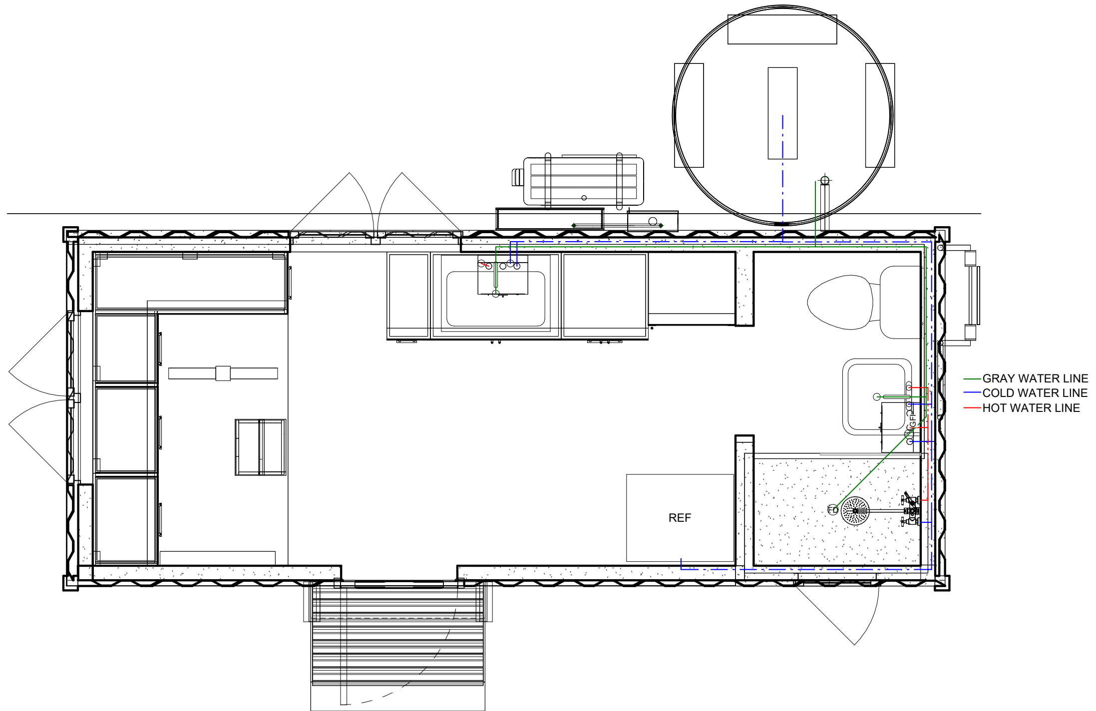
① Bottom of container PLUMBING 1/2" = 1'-0"
