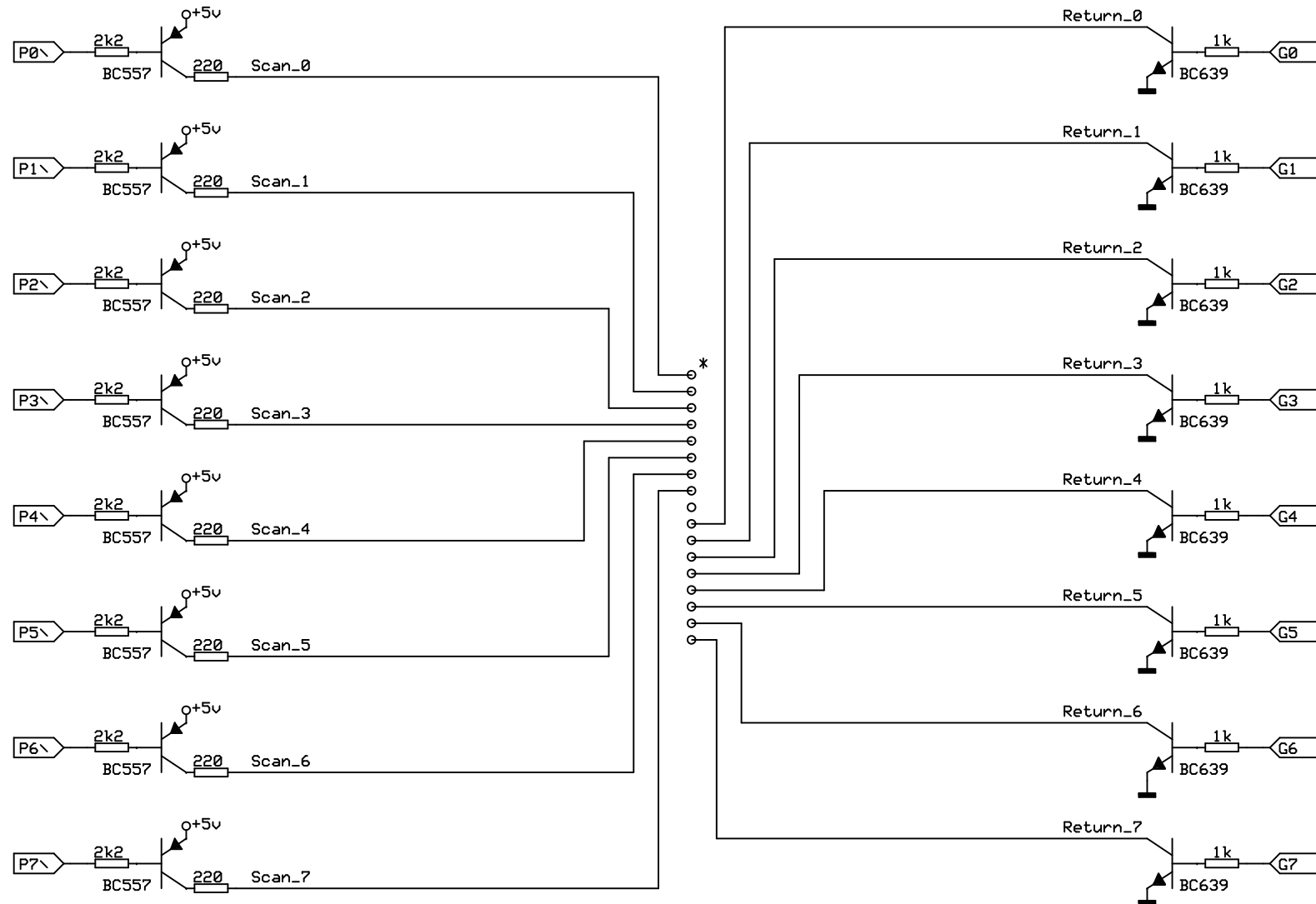
Scan Line Drivers
