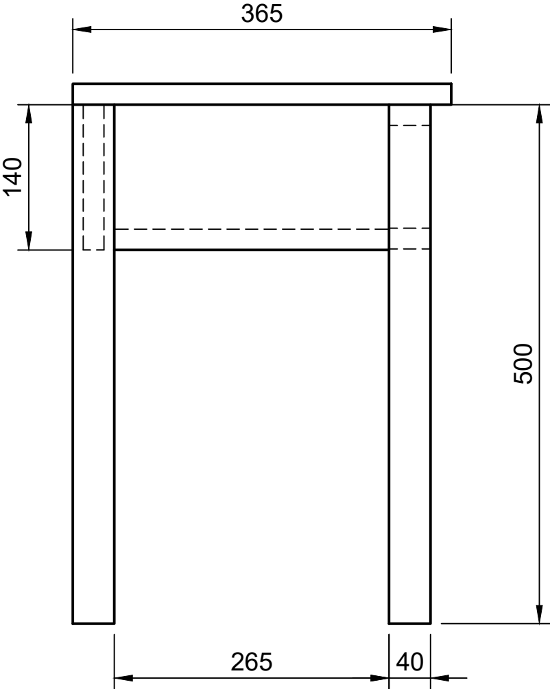
SIDE VIEW
