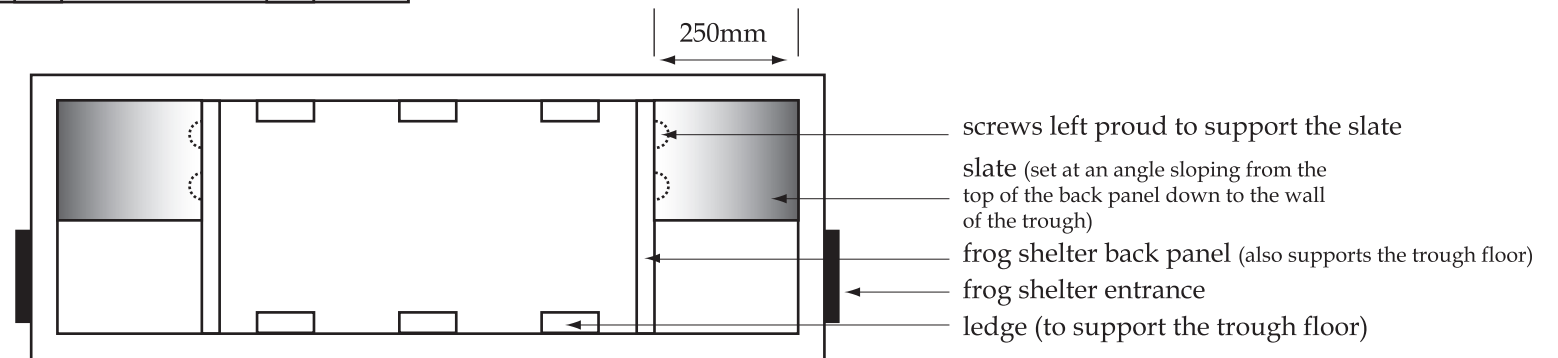
top view
